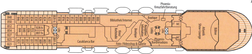
Deck 08 Salon-Deck
